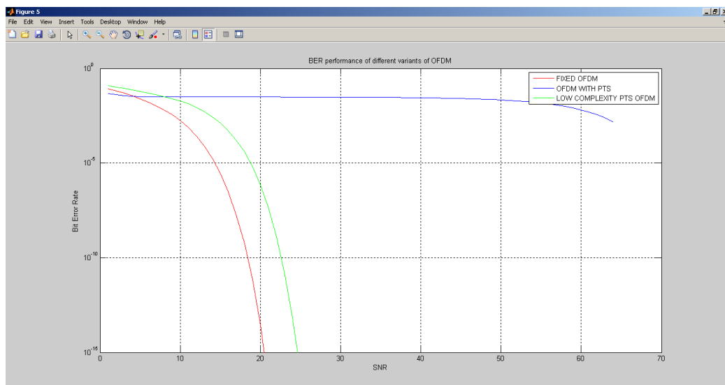
Figure 5: Graph showing comparative analysis for N=64
