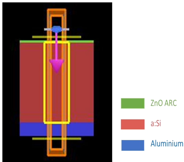
Figure 3: View of a: Si unit solar cell in FDTD Analysis
