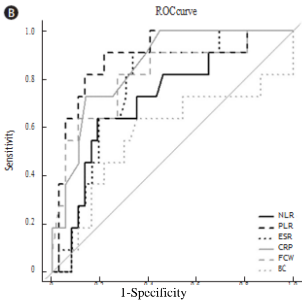
Figure 2: ROC curve showing the diagnostic performance of NLR, PLR, and FC. (A) In the ROC curve, the optimal cut off value for NLR and PLR for detecting UC was 2.26 (sensitivity 54.2%; specificity 90.6%; AUC0.774, 95% CI0.690–0.859) and 179.8 (sensitivity 35.4%; specificity 90.6%, AUC0.654, 95% CI0.556–0.753). (B) The optimal cutoff value for NLR, PLR, and FC for differentiating UC
