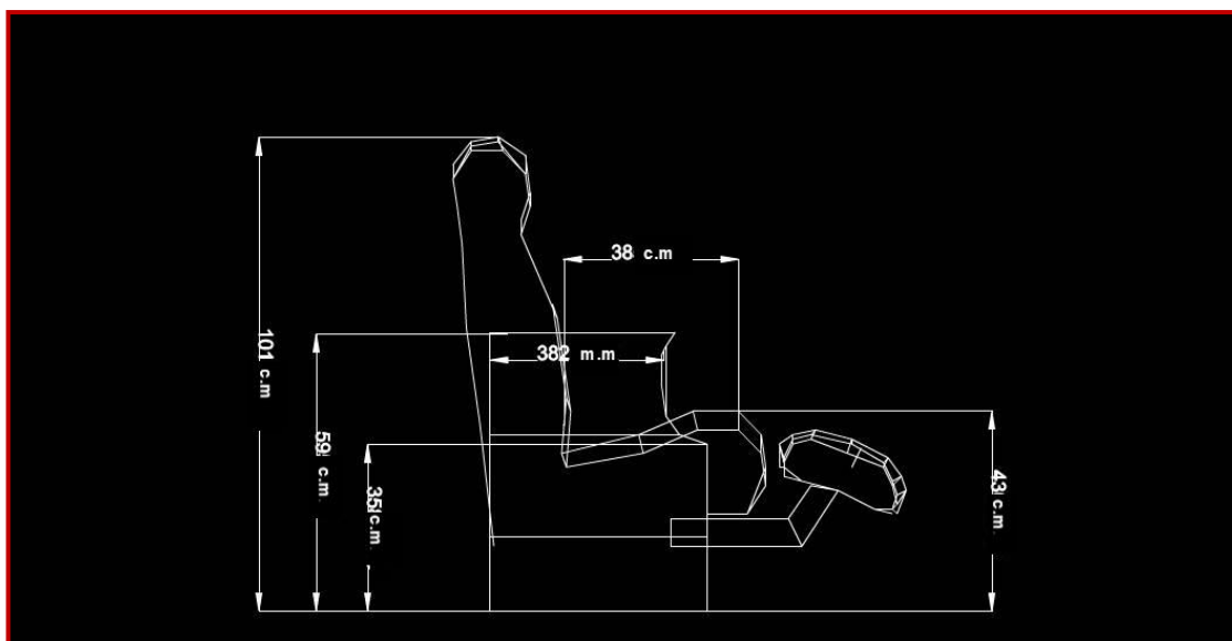
Plate 1: Side view of relaxing chair through the CAD sketching
