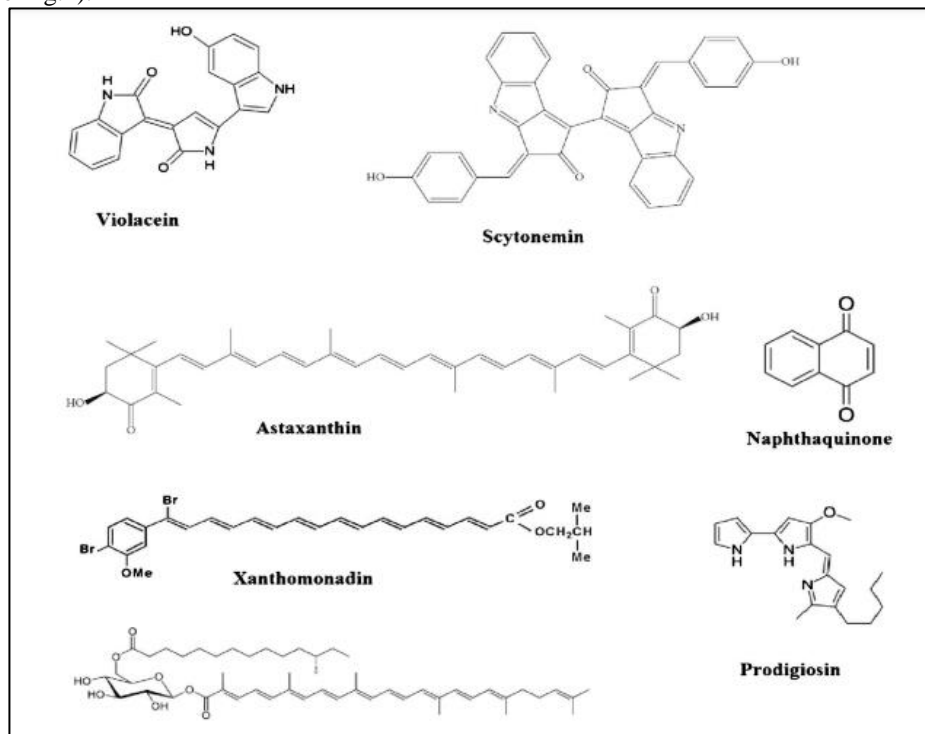
Figure 4: Chemical structures of some pharmacologically active microbial pigments
