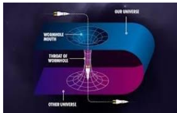
Figure 2: Illustration of a Wormhole in a 2-Dimensional Universe. [7]
