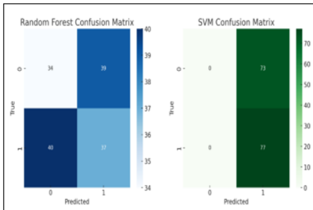
Figure 2: Confusion Matrix
