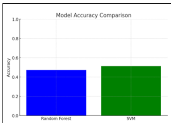
Figure 3: Accuracy Comparison
