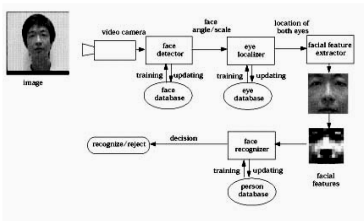
Figure 1: Face Recognition System [5]
