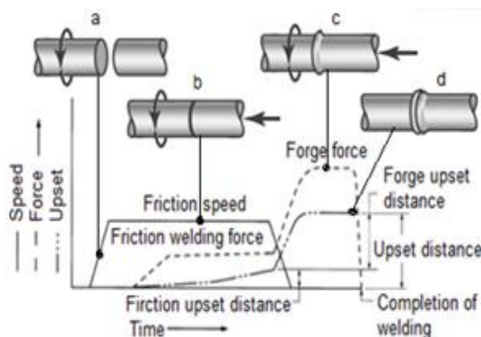
Figure 1: Friction welding
