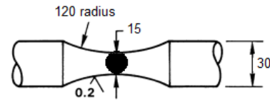
Figure 4: Specimen of fatigue test (all dimensions are in mm).
