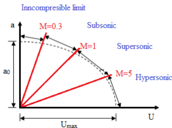
Figure 2.4: Showing steady flow adiabatic ellipse
