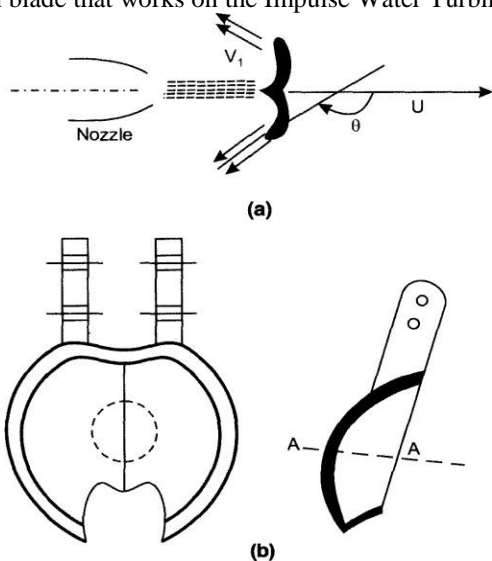
Figure 4: Pelton blade.[4]
