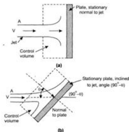
Figure 1: Flow blows flat blade [4] a) Vertical blade position b) Tilt blade position.
